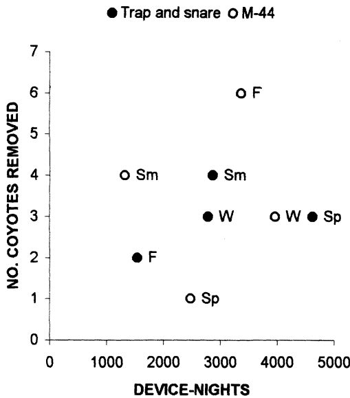
Fig. 1. Capture success versus removal effort associated with stationary devices during 4 seasons: winter (W; Jan–Mar), spring (Sp; Apr–Jun), summer (Sm; Jul–Sep), and fall (F; Oct–Dec), illustrating no relation in the observed range of effort expended, Hopland Research and Extension Center, Mendocino County, California, April 1994–October 1995.
